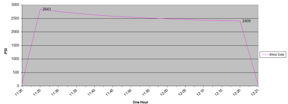
▲ AGC / HGC Cylinder Test Stand
